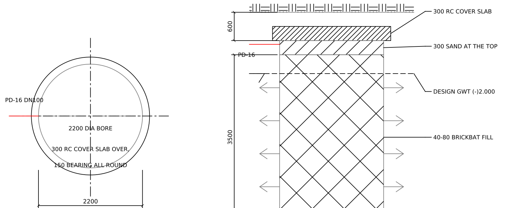
5 SOAK PIT SK-01 - PLAN 1 : 50 SK-02 IS IDENTICAL 6 SOAK PIT SK-01 - SECTIONAL ELEVATION 1 : 50 2200 DIA x 3500 EFFECTIVE, IS 2470 (Pt 2):1985
