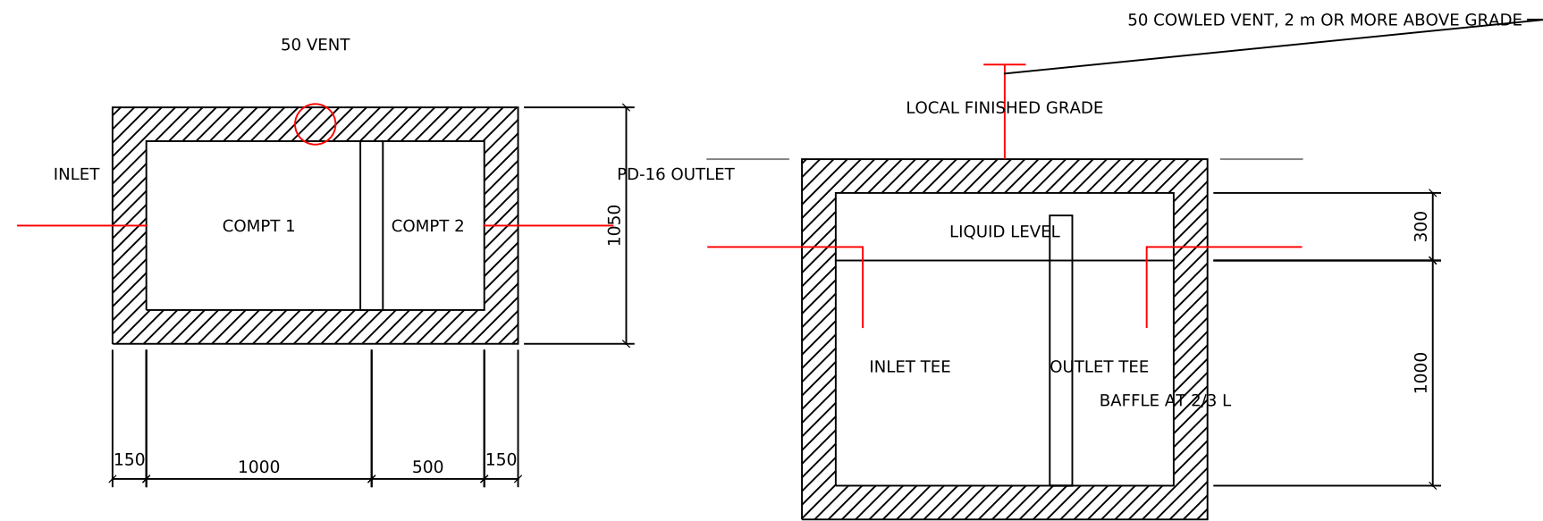
3 SEPTIC TANK ST-01 - PLAN 1 : 30 1500 x 750 LIQUID, 150 WALLS 4 SEPTIC TANK ST-01 - SECTIONAL ELEVATION 1 : 30 IS 2470 (Pt 1):1985
