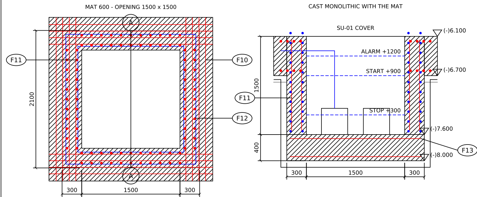
1 SUMP PIT SU-01 - REINFORCEMENT PLAN 1 : 35 BAY 5, X 11068 - 12568, Y 900 - 2400 2 SUMP PIT SU-01 - SECTIONAL ELEVATION A-A 1 : 35 3.375 m3, INVERT (-)7.600
