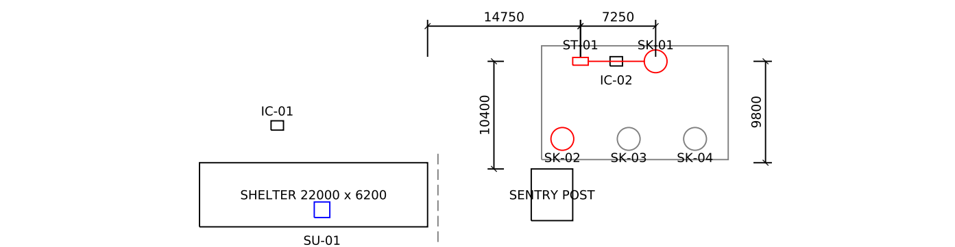
7 KEY PLAN - EXTERNAL WORKS LOCATION 1 : 500 EAST OF THE SHELTER AND NORTH OF THE SENTRY POST
